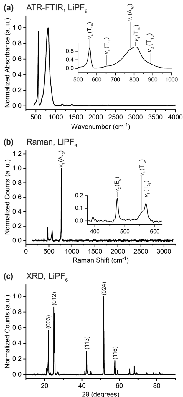
Fig. 5 (a) ATR-FTIR, (b) Raman, and (c) XRD data for lithium hexafluorophosphate (LiPF 6 ). Peaks are identified from the literature: (a,b) from Kock et al. 72 and (c) from Masoud et al. 124 .
